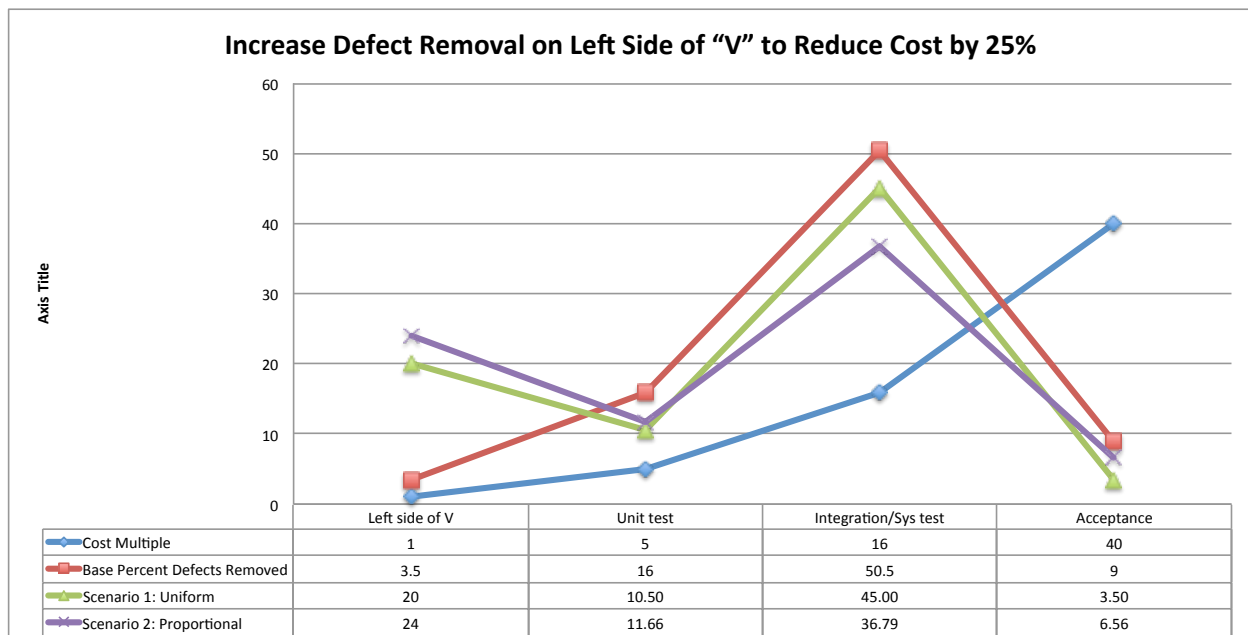
Figure 16. How Much Improvement in Defect Removal on Left Side of "V" is needed to Reduce Cost/Effort by 25 Percent
